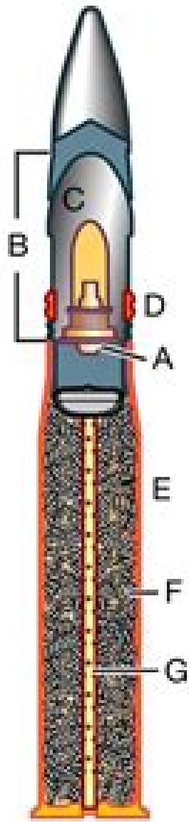
fixed ammunition
