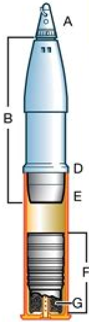
semifixed ammunition
