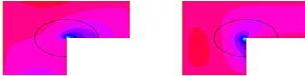
Figure 4: Real part \Re(\mathbf{y}_{S_r}^1) and \Re(\mathbf{y}_{S_z}^1) of the singular basis for k = 1 , r and z components.
