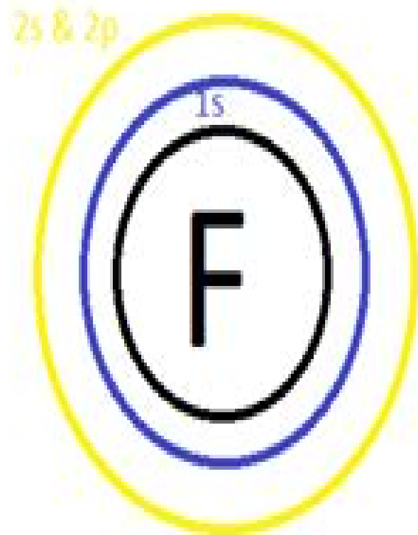
Normal Flourine Atom
