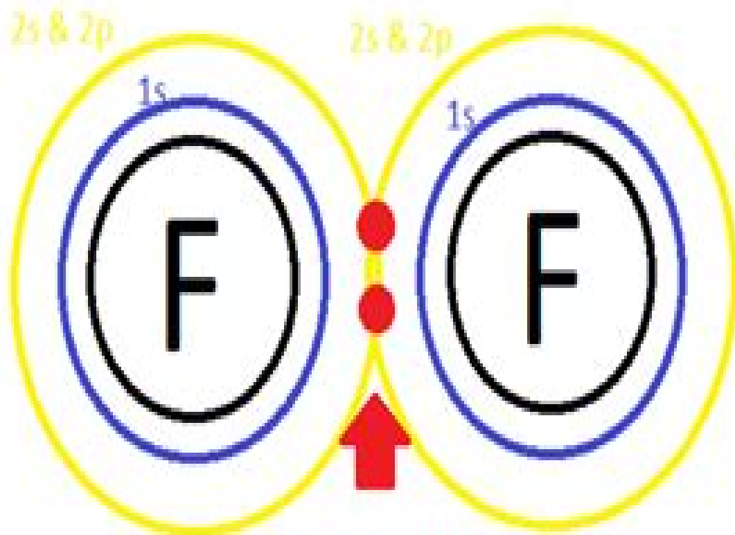
Flourine Atoms Covalently Bonded
