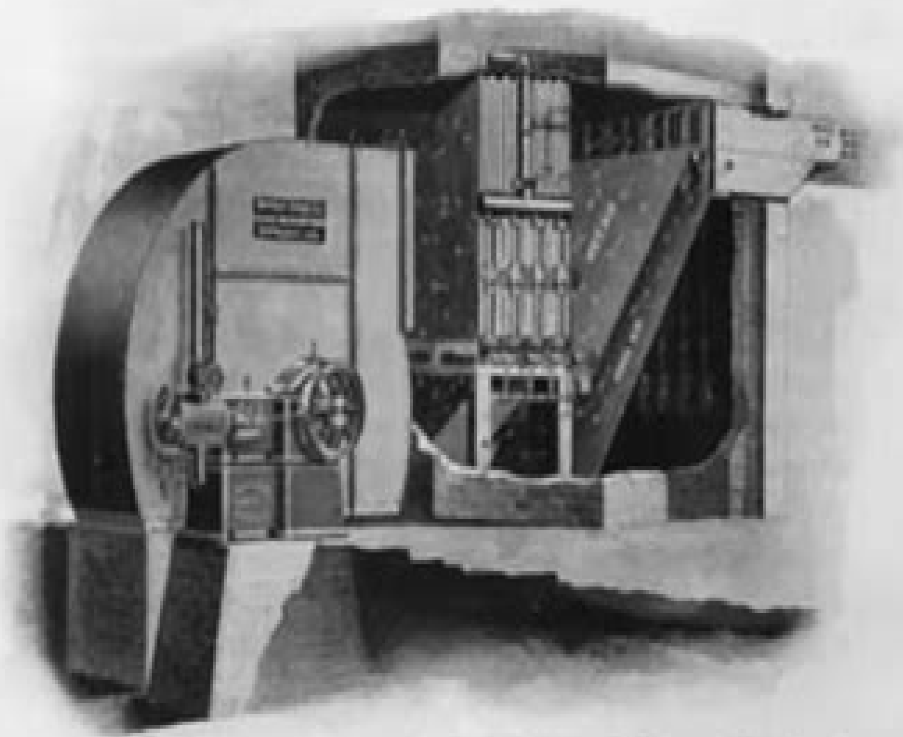
Three-Quarter Housing Fan, Left-Hand Top Horizontal Discharge, Blowing Air Through and Underneath Heater into Brick Plenum Chamber
