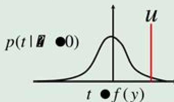
Classical T-test
