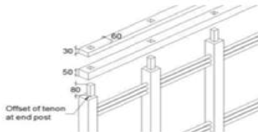
Figure 4. quinchá mortice and tenon detail [19]
