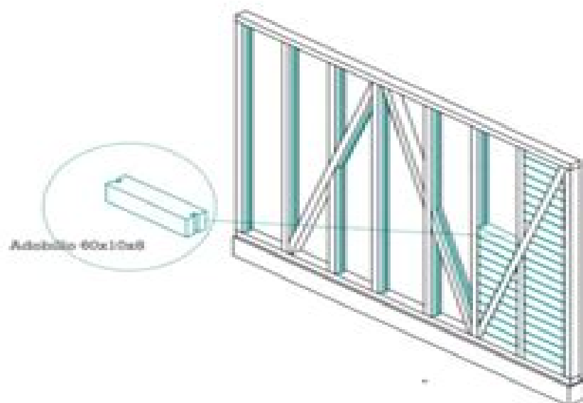
Figure 5. diagram of adobillo constructive system mounting [13]
