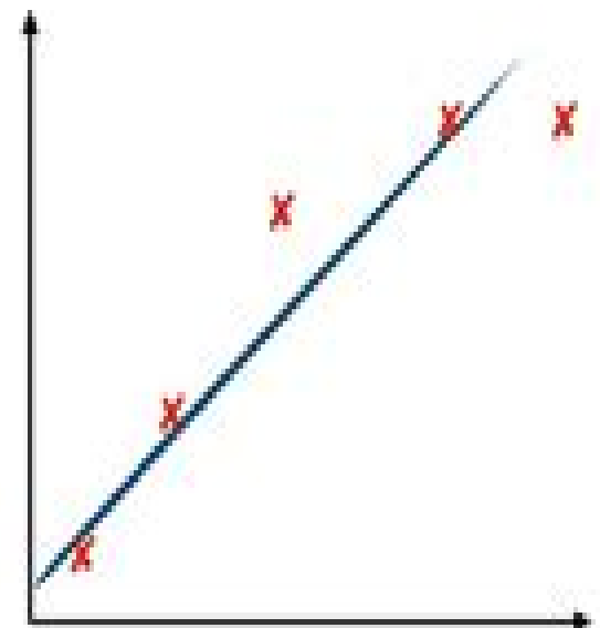
Machine Learning
