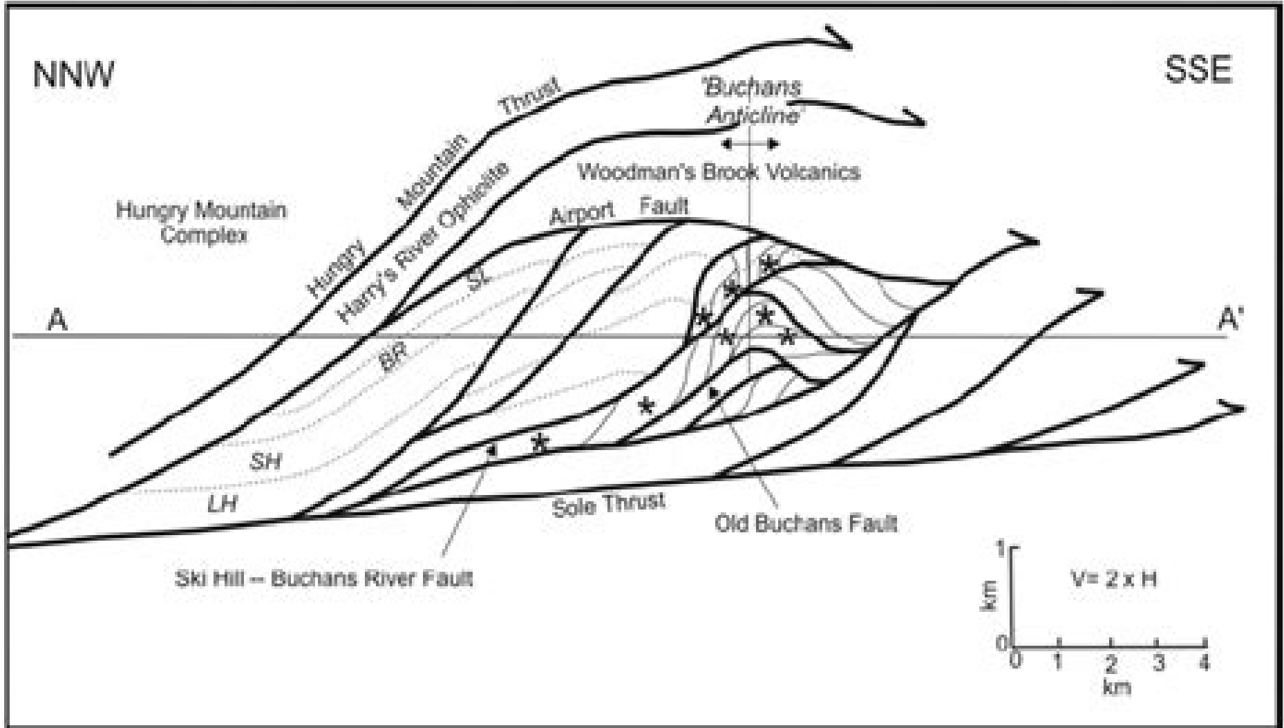
Figure 30. Schematic NNW-SSE cross-section showing the geometry of the Buchans thrust stack, modified slightly from Calon and Greene (1987). LH = Lundberg Hill Formation; SH = Ski Hill Formation; BR = Buchans River Formation; SL = Sandy Lake Formation. Asterisks indicate positions of the main Buchans orebodies. See Figure 28 for location of cross section.
