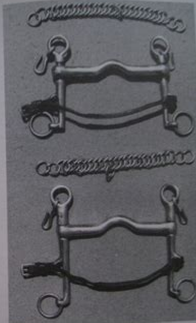
72 Slide mouth Weymouth bit, compare with 50 (top). Weymouth bit with up sliding action (bottom).
