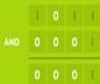
Bitmask
